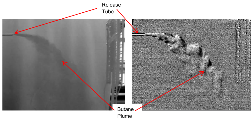
Figure 2 Two FLIR GasCam images of an indoor butane release, showing standard resolution and high resolution
