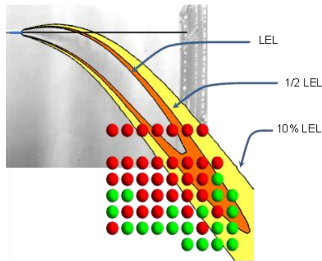
Figure 3 Comparison of hydrocarbon camera image (greyscale) and predicted mean gas concentrations from the CFD model (coloured contours) with the ignition data, where ● indicates successful ignition and ● indicates no ignition. The CFD results shown here used a 0.1 m/s wind flowing in the same direction as the gas release
