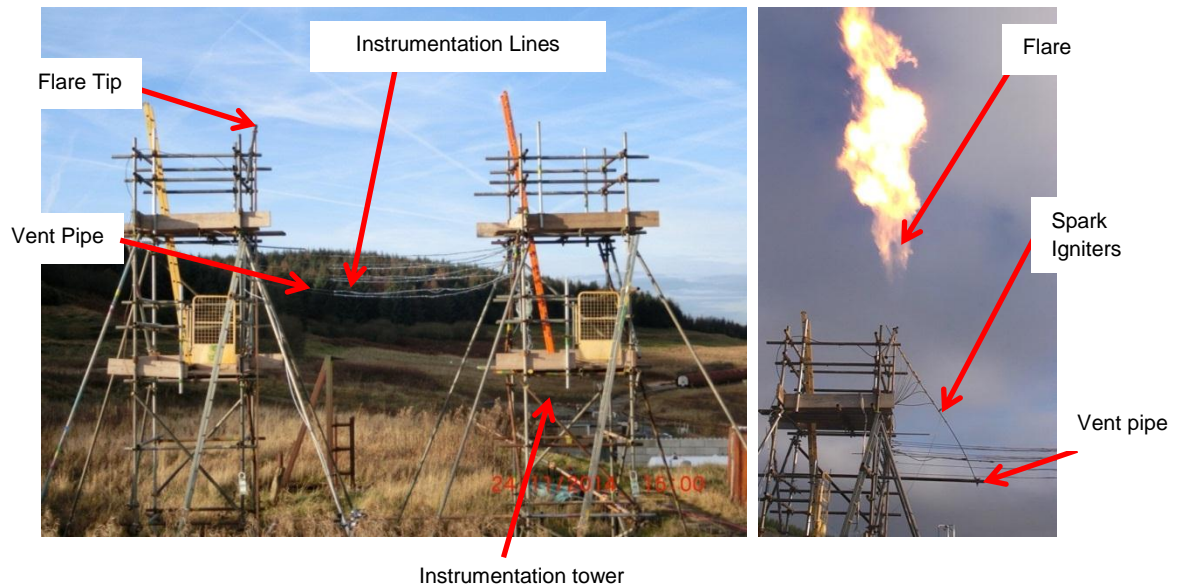
Figure 4 Photos of the outdoor gas dispersion experimental rig
