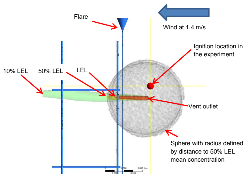
Figure 5 Side view of predicted butane gas cloud in the first outdoor gas dispersion experiment
