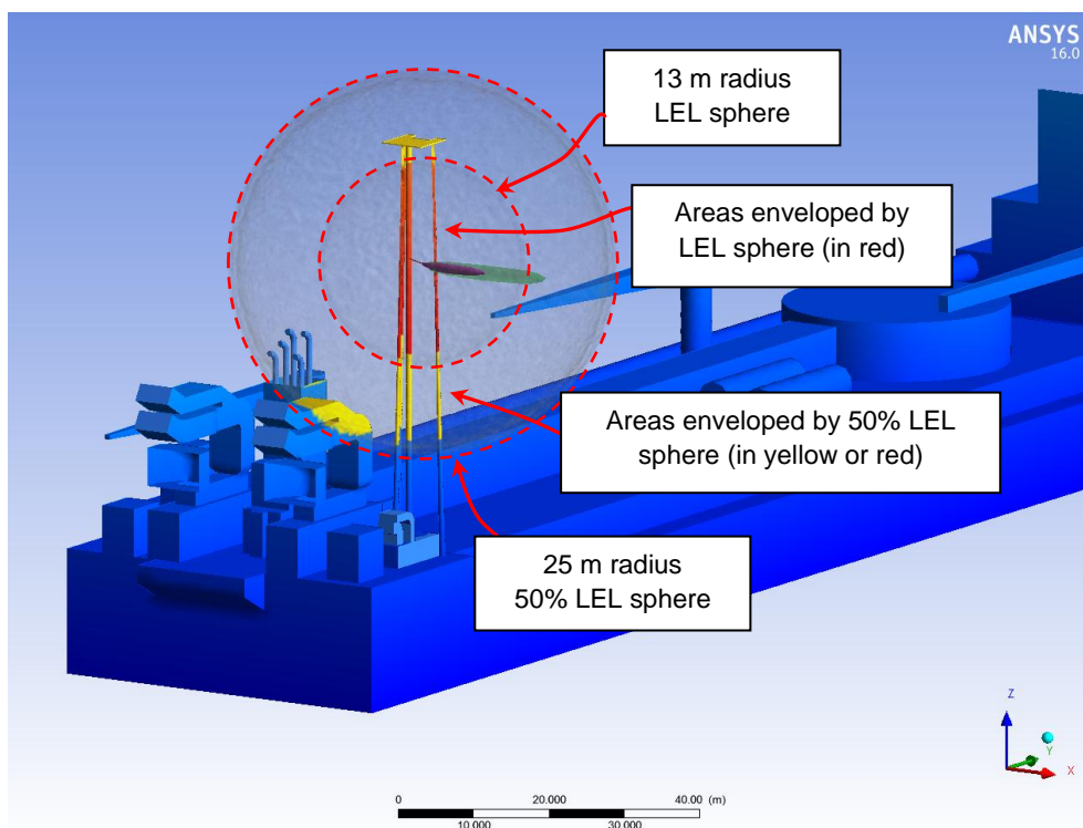
Figure 6 Side view of the predicted 50% LEL and LEL clouds for second GP3 ignition incident
